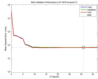
Fig. 4. MSE vs Epochs for MFNN Predictor
