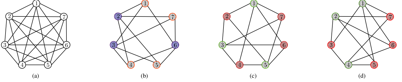
Figure 2: Figure (a) shows the hypergraph K_7 which is the complete graph on 7 vertices. It requires 7 colors for a conflict-free coloring, thus \mathcal{X}_{CF}(K_7) = 7 . The three figures (b),(c) and (d) depict a collection of 1-fold conflict-free colorings, each figure corresponding to one coloring using 2 colors. Note that only those edges satisfied by the coloring are represented in (b), (c), and (d). In (b), the two color classes are \{1, 4, 5, 7\} and \{2, 3, 6\} . In (c), they are \{2, 4, 6, 7\} and \{1, 3, 5\} and in (d) they are \{1, 2, 4\} and \{3, 5, 6, 7\} . It can be checked that each edge of K_7 is conflict-free in at least one of these colorings. Thus \alpha_{CF}(\mathcal{H}) \leq 6 < \mathcal{X}_{CF}(\mathcal{H}) .
