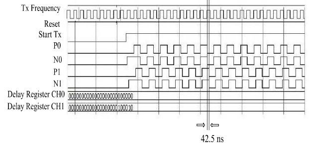
Fig. 13: Gate level simulation results in Design Compiler.
