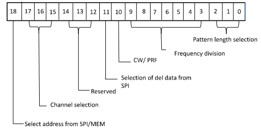
Fig. 4: Bit structure of configurable control register
