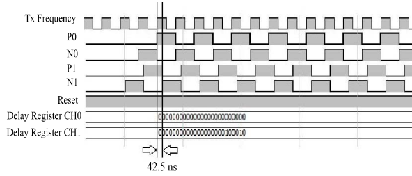
Fig. 9: Simulation result of Tx beamforming design.
