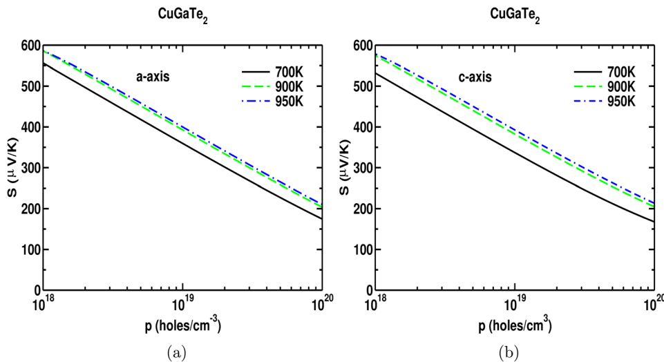
FIG. 3. Thermopower variation with hole concentration along the (a) a-axis and (b) c-axis at different temperatures for CuGaTe 2 .
