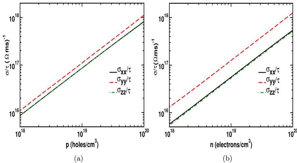
FIG. 10. Variation of the ratio (\sigma/\tau) with (a) hole concentration and (b) electron concentration along the three lattice directions for \text{CuSbS}_2 at T = 300 \text{ K} .
