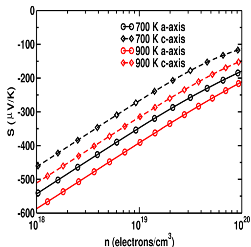
FIG. 5. Thermopower variation with electron concentration along the a- and c-axes at different temperatures for CuGaTe 2 .
