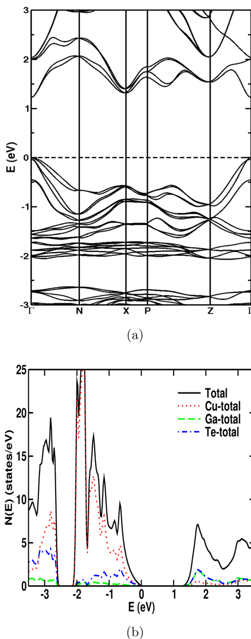
FIG. 1. Calculated (a) band structure and (b) density of states of CuGaTe 2 . The energy zero corresponds to the valence band maximum.
