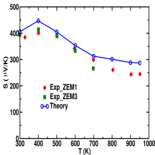
FIG. 4. The variation of the calculated thermopower as a function of temperature for CuGaTe 2 (see text for explanation) compared with available experimental data (Ref. 26) for two different samples.
