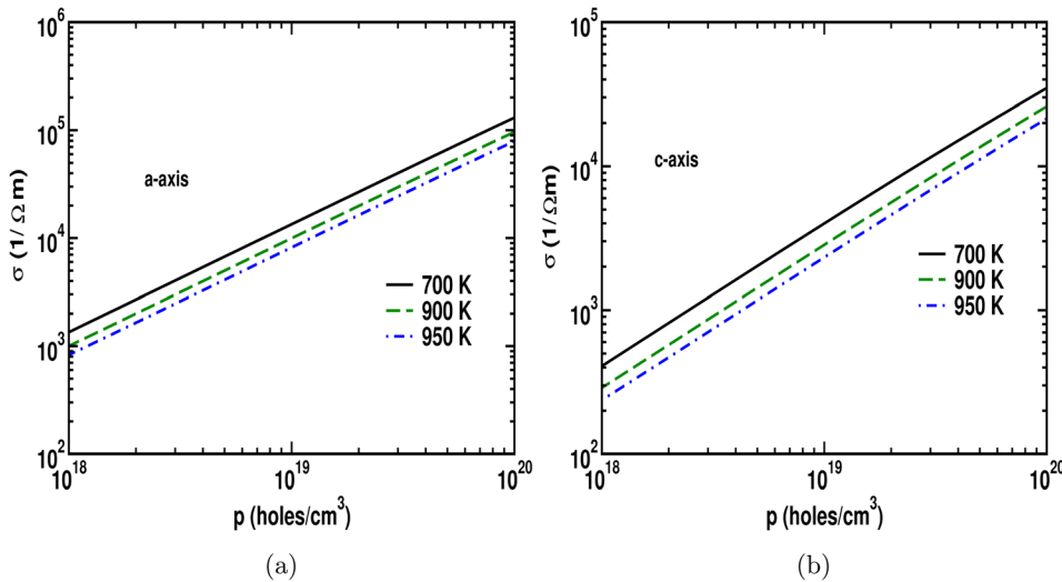
FIG. 8. Electrical conductivity variation with hole concentration along the (a) a-axis and (b) c-axis at different temperatures for CuGaTe 2 .
