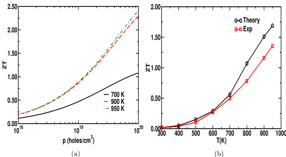
FIG. 12. Calculated figure of merit of \text{CuGaTe}_2 as function of (a) the hole concentration for three different temperatures and (b) temperature for the experimental carrier density and compared to experiment. 26
