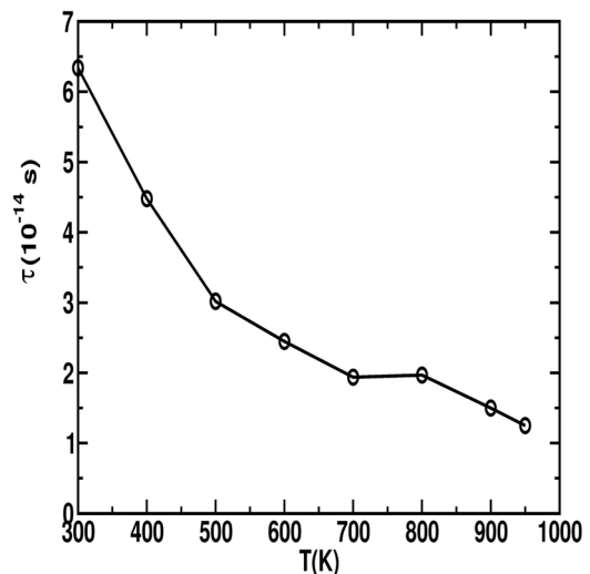
FIG. 7. Temperature variation of the relaxation time \tau of \text{CuGaTe}_2 , estimated as explained in text.
