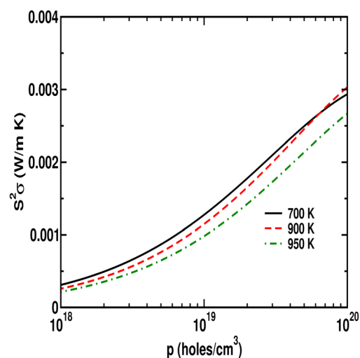
FIG. 9. Variation of the power factor with hole concentration for CuGaTe 2 .
