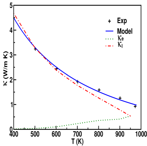
FIG. 11. The experimental 26 thermal conductivity of \text{CuGaTe}_2 (crosses) compared with the fitting expression (see text—full line, blue). The electronic (dashed) and lattice contributions (dashed-dotted) are shown separately.
